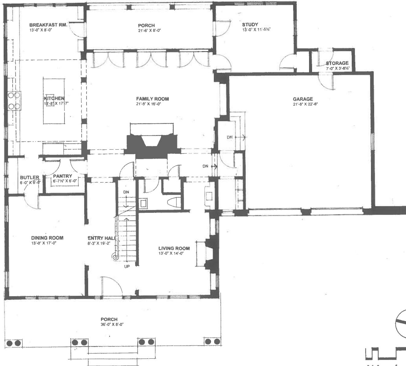
FIRST FLOOR PLAN 1/4" = 1'-0"
